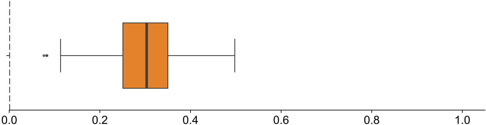
McGrath Categorical
