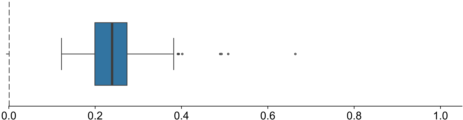
Task Space
