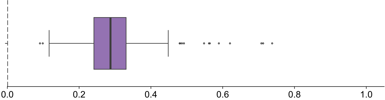
Laughlin Subspace
